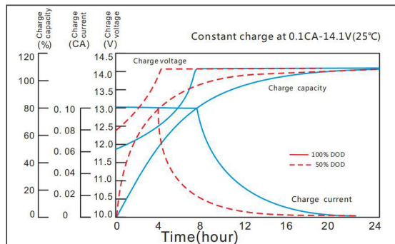
Charging characteristic
